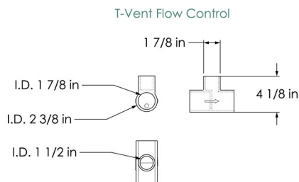
T-Vent Flow Control
